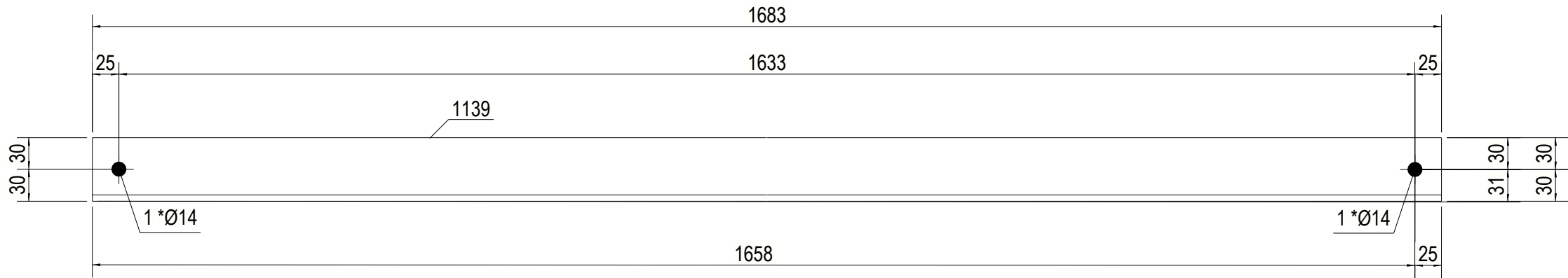
FRONT VIEW
